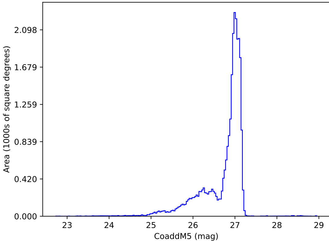
too_5_1v3.4_10yrs r: CoaddM5
