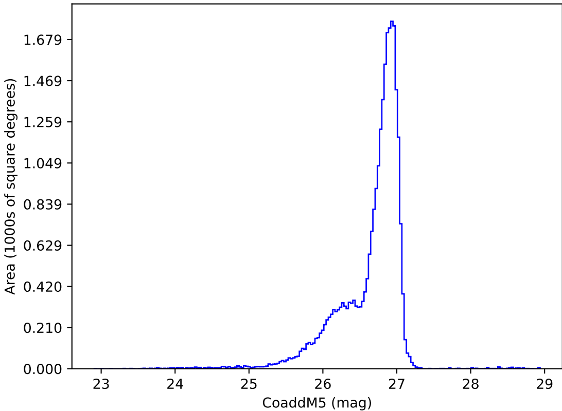
too_5_1v3.4_10yrs g: CoaddM5
