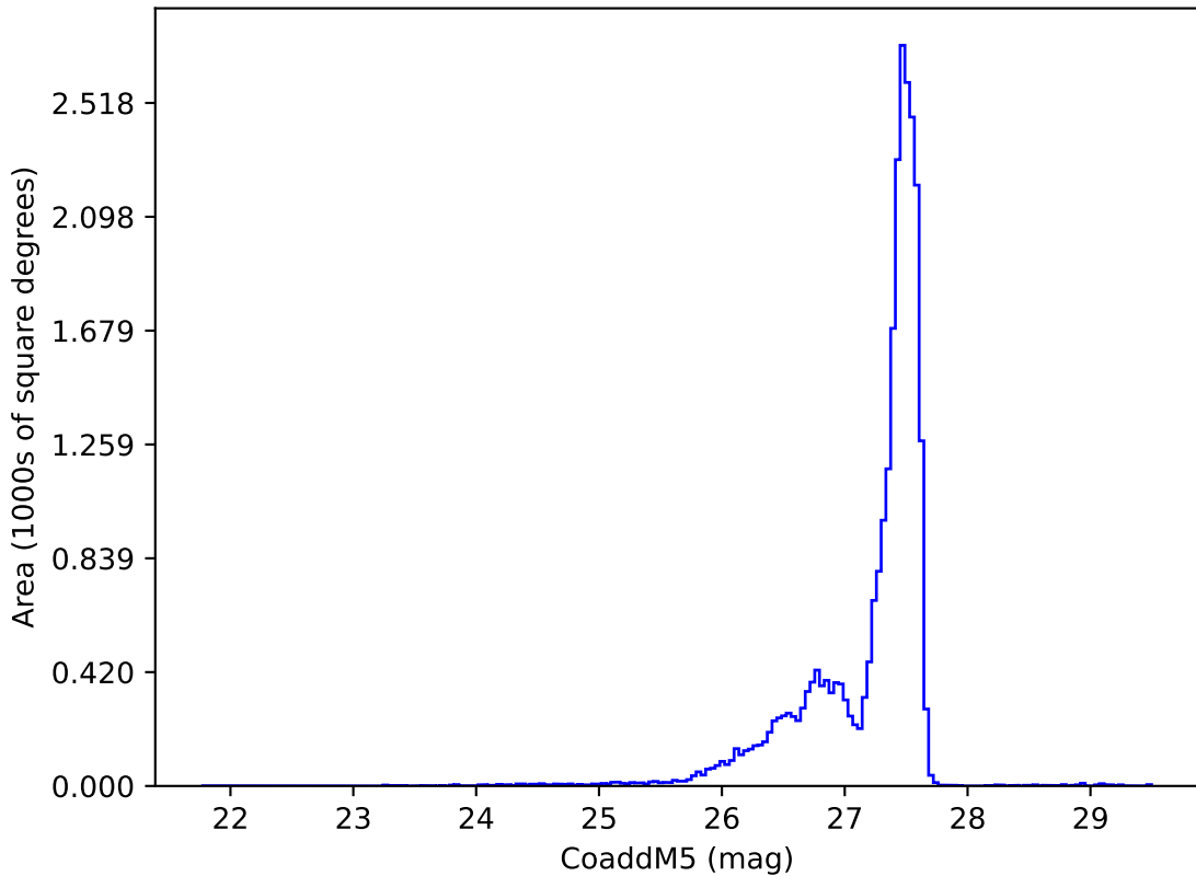
too_5_1v3.4_10yrs : CoaddM5
