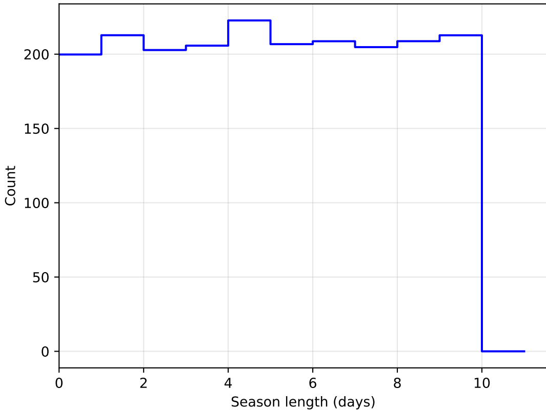
too_5_1v3.4_10yrs DD:XMM_LSS all bands: SeasonLength
