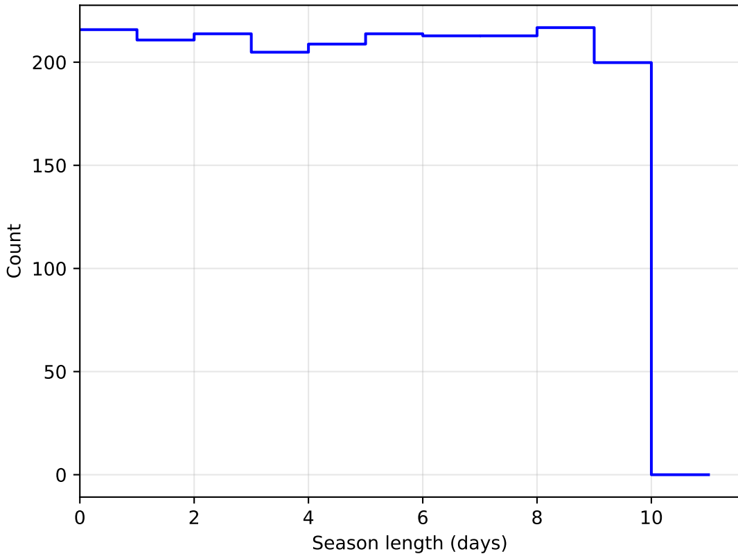
too_5_1v3.4_10yrs DD:ECDFS all bands: SeasonLength
