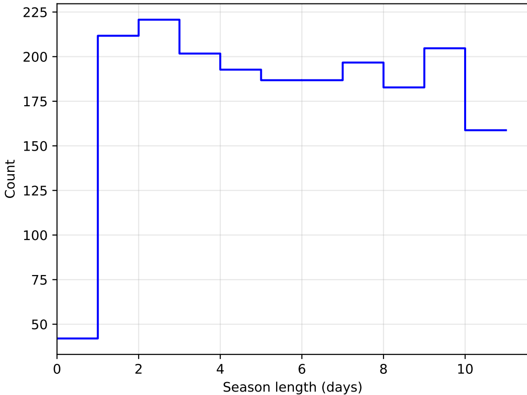
too_5_1v3.4_10yrs DD: COSMOS all bands: SeasonLength
