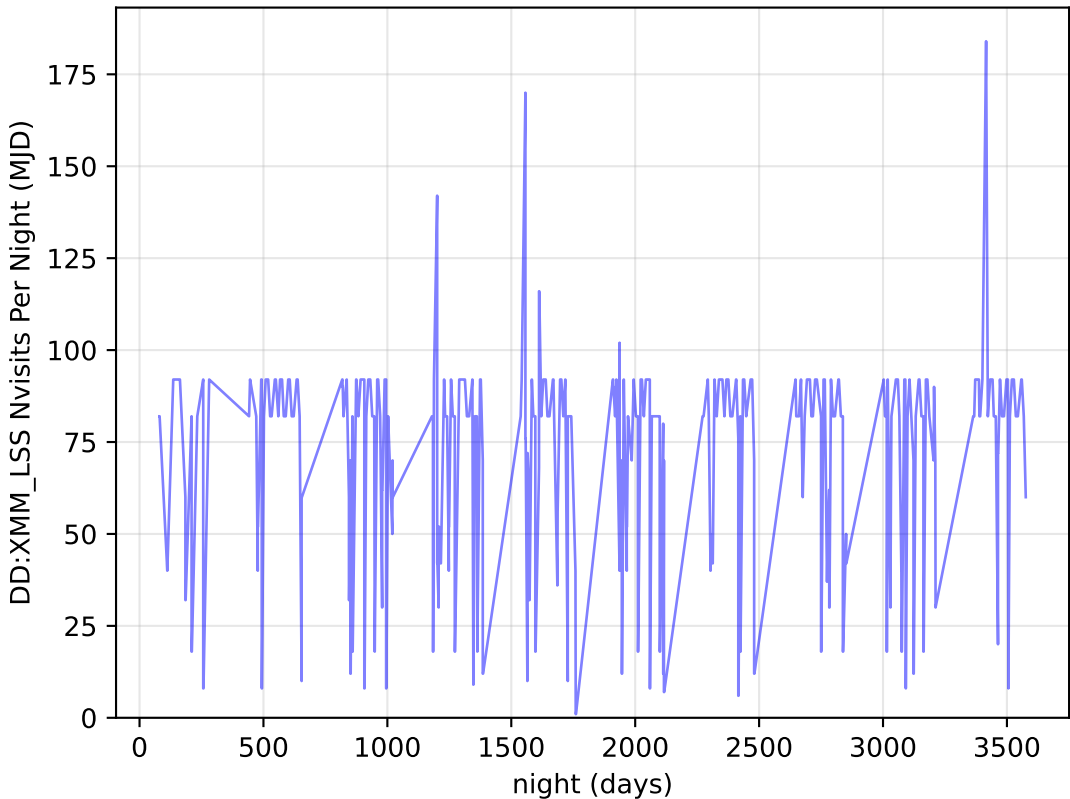
too_5_1v3.4_10yrs all bands: DD:XMM_LSS Nvisits Per Night
