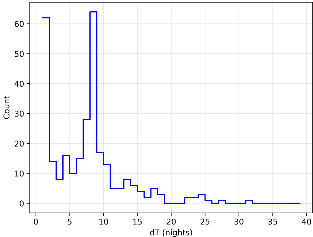
too_5_1v3.4_10yrs all bands: DD:XMM_LSS Delta Nights Histogram
