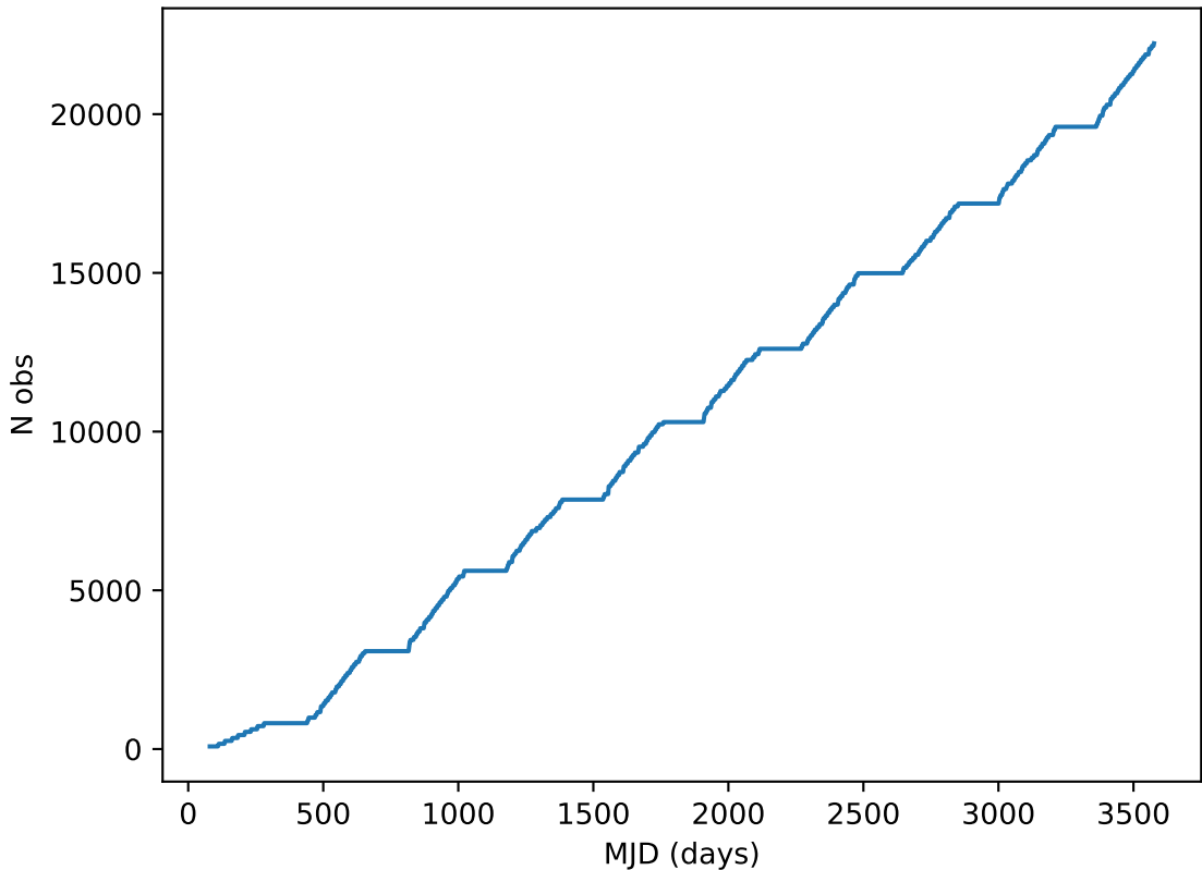
too_5_1v3.4_10yrs all bands: DD:XMM_LSS Cumulative NVisits
