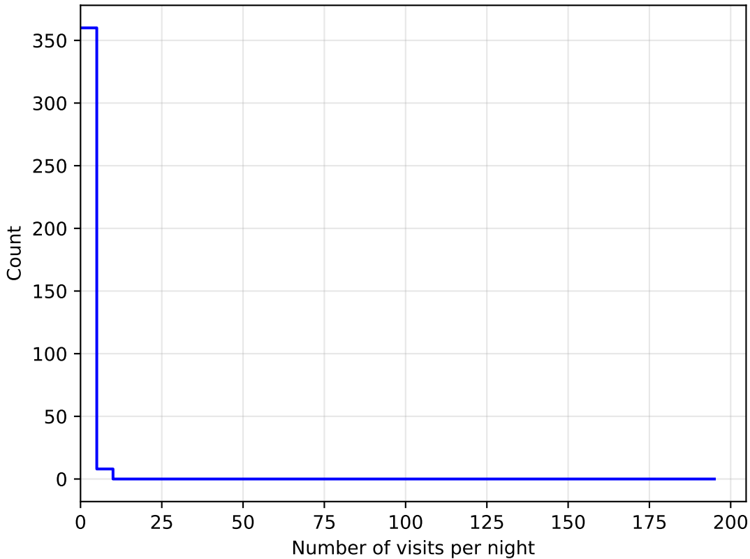
too_5_1v3.4_10yrs all bands: DD:WFD NVisitsPerNight
