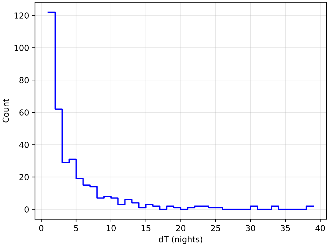
too_5_1v3.4_10yrs all bands: DD:WFD Delta Nights Histogram
