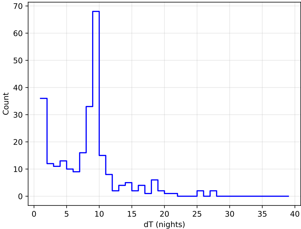
too_5_1v3.4_10yrs all bands: DD:ELAISS1 Delta Nights Histogram
