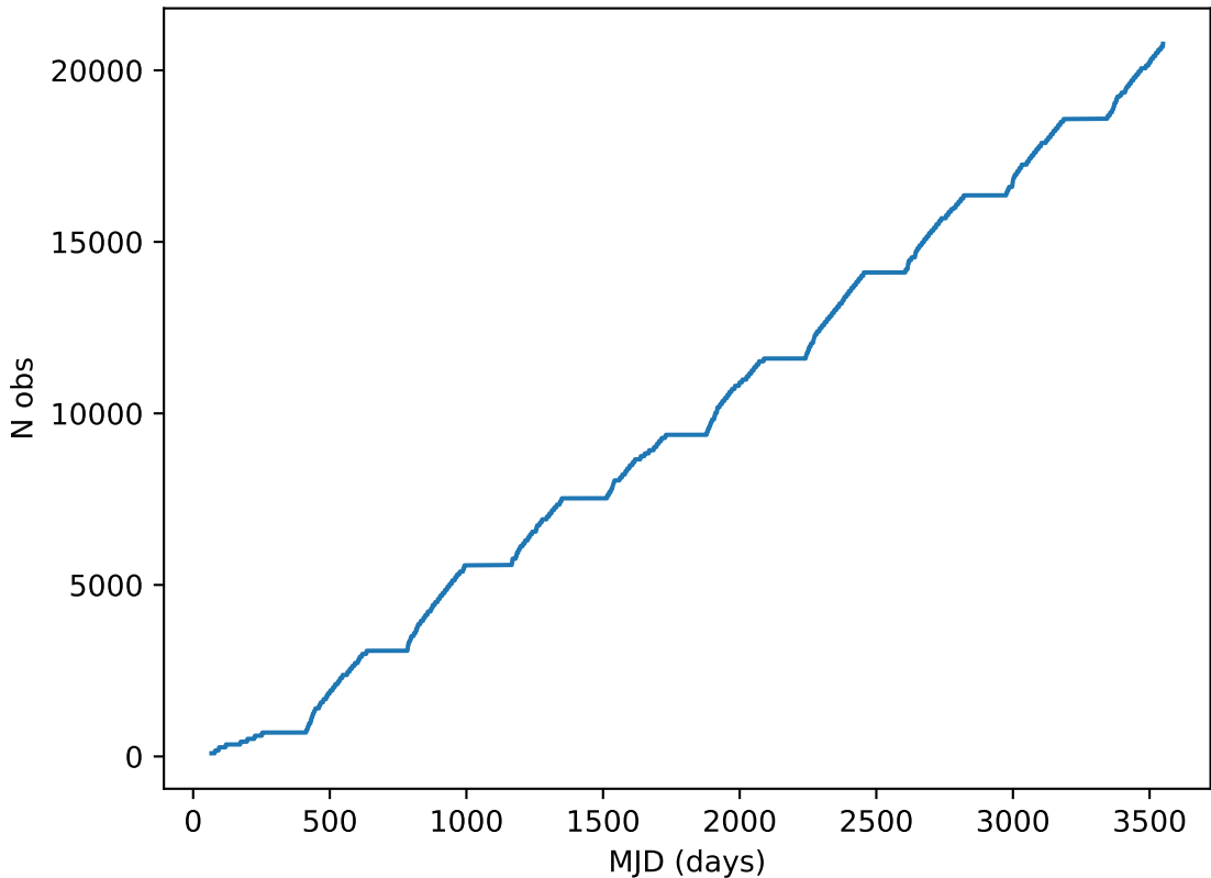
too_5_1v3.4_10yrs all bands: DD:ELAISS1 Cumulative NVisits
