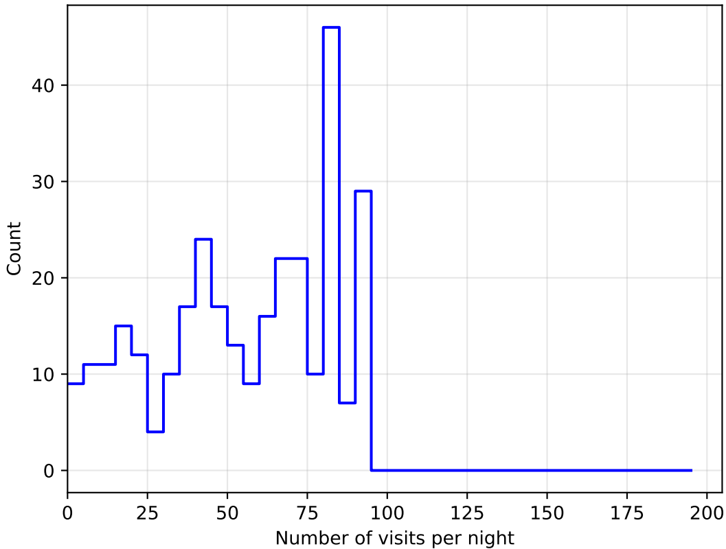
too_5_1v3.4_10yrs all bands: DD:EDFS NVisitsPerNight
