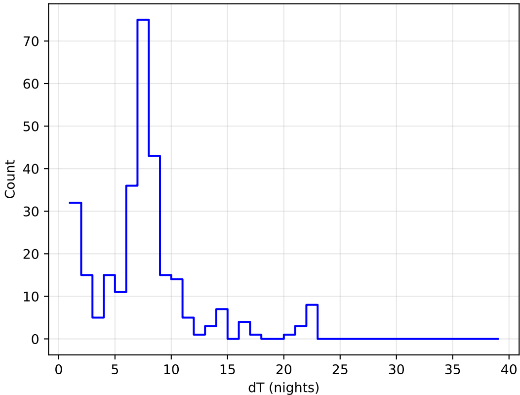
too_5_1v3.4_10yrs all bands: DD:EDFS Delta Nights Histogram
