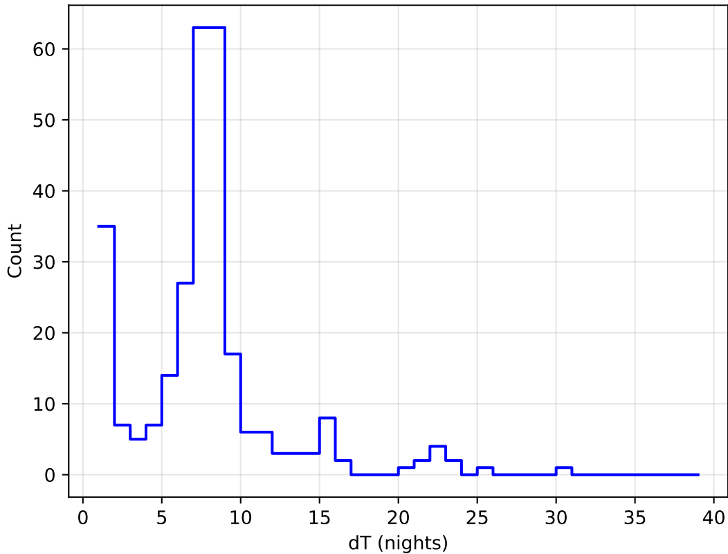
too_5_1v3.4_10yrs all bands: DD:ECDFS Delta Nights Histogram
