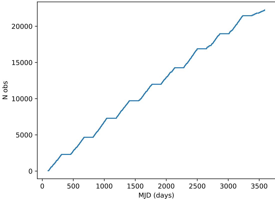
too_5_1v3.4_10yrs all bands: DD:ECDFS Cumulative NVisits
