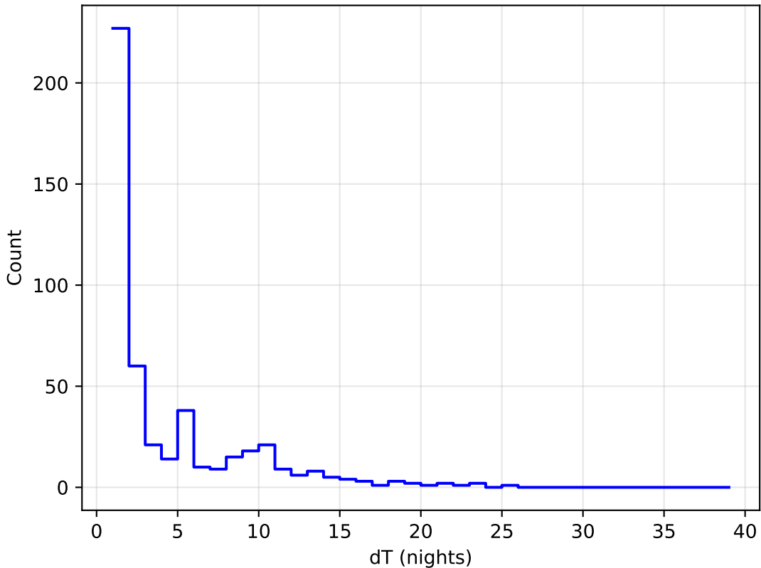
too_5_1v3.4_10yrs all bands: DD: COSMOS Delta Nights Histogram
