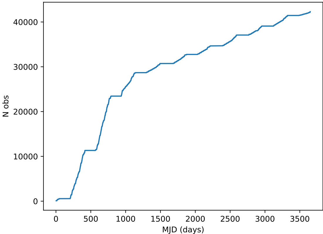
too_5_1v3.4_10yrs all bands: DD: COSMOS Cumulative NVisits
