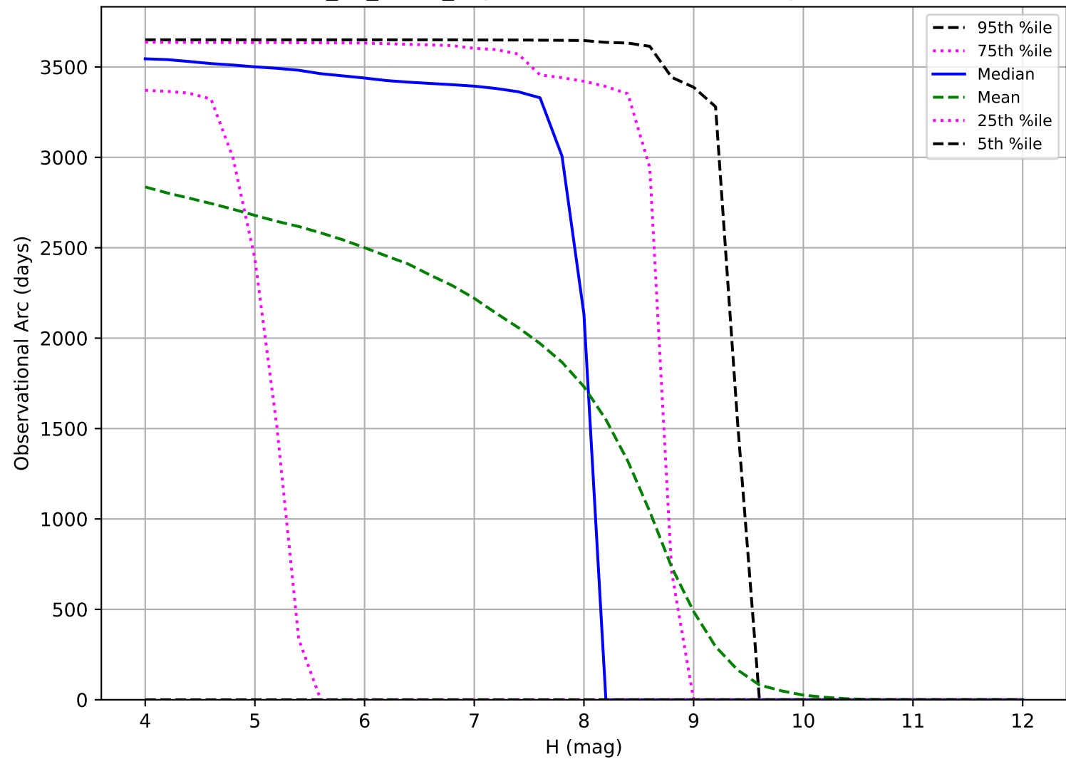
too_10_4v3.4_10yrs: Observational Arc Length TNO
