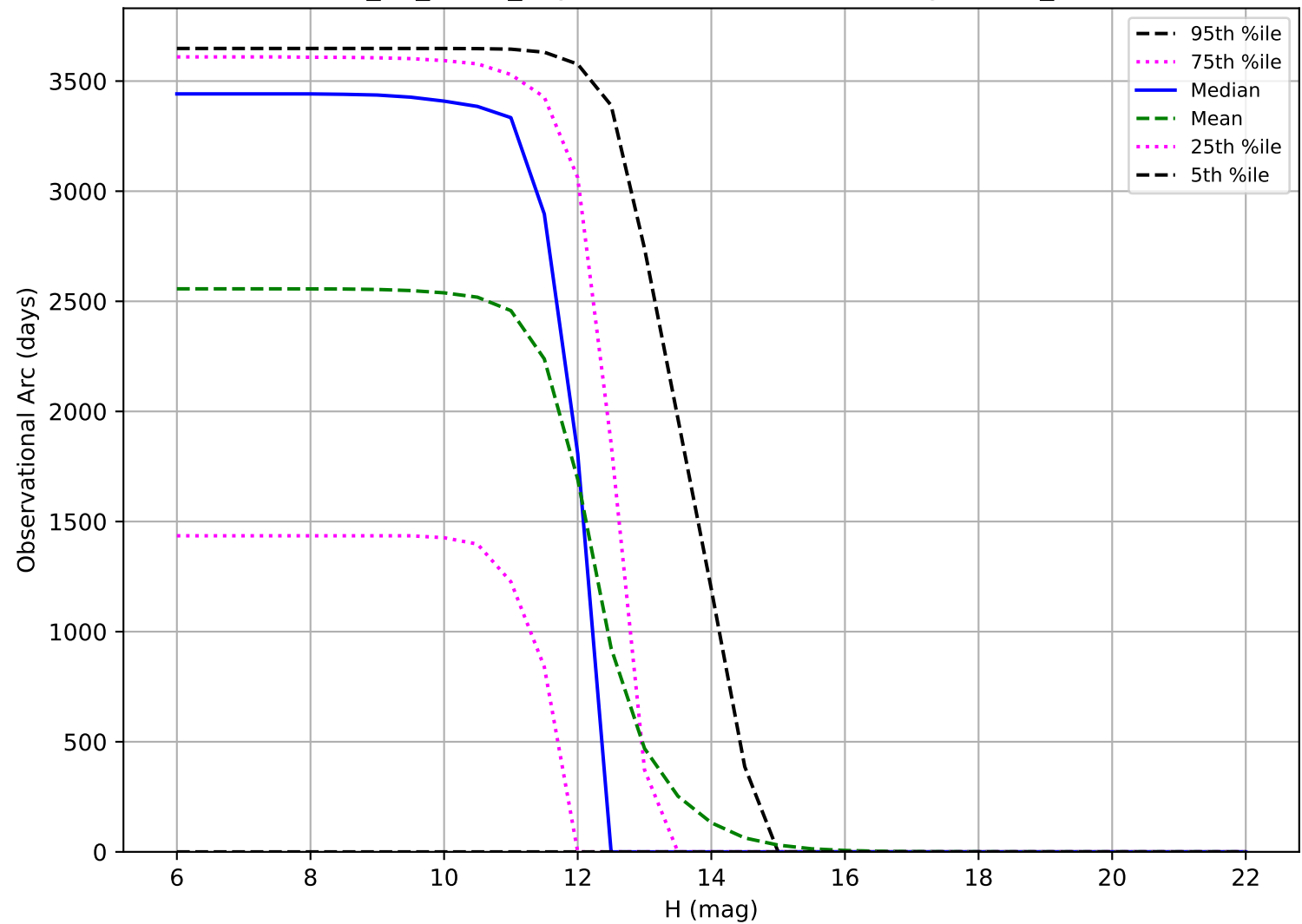
too_10_4v3.4_10yrs: Observational Arc Length OCC_r20
