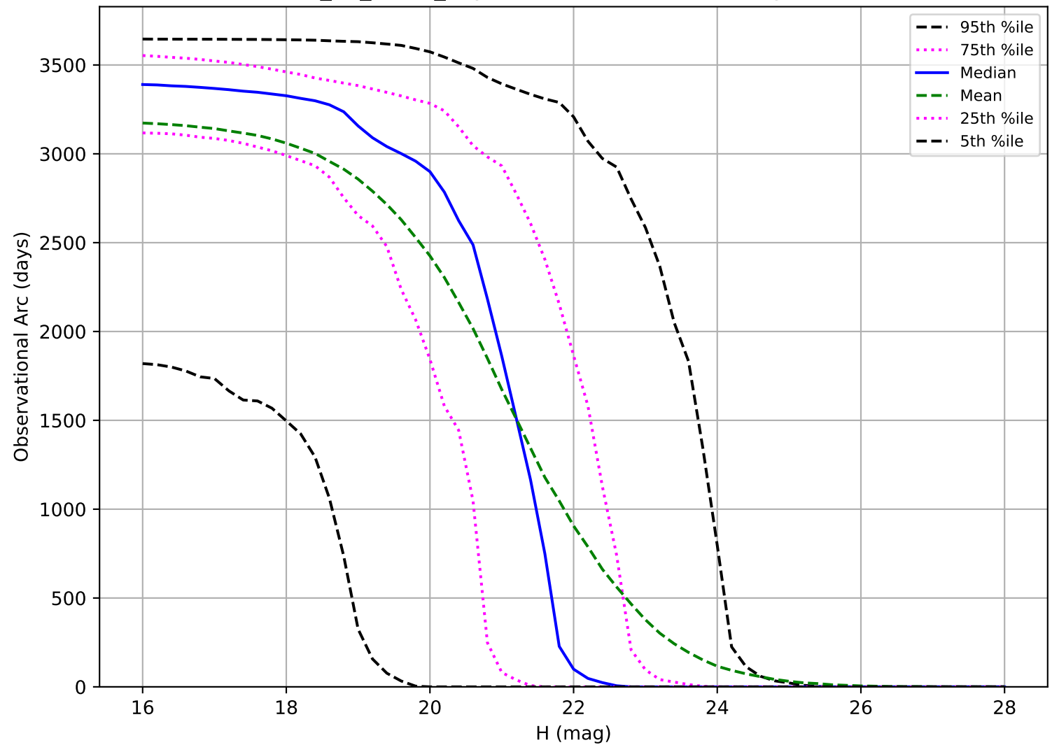
too_10_4v3.4_10yrs: Observational Arc Length NEO
