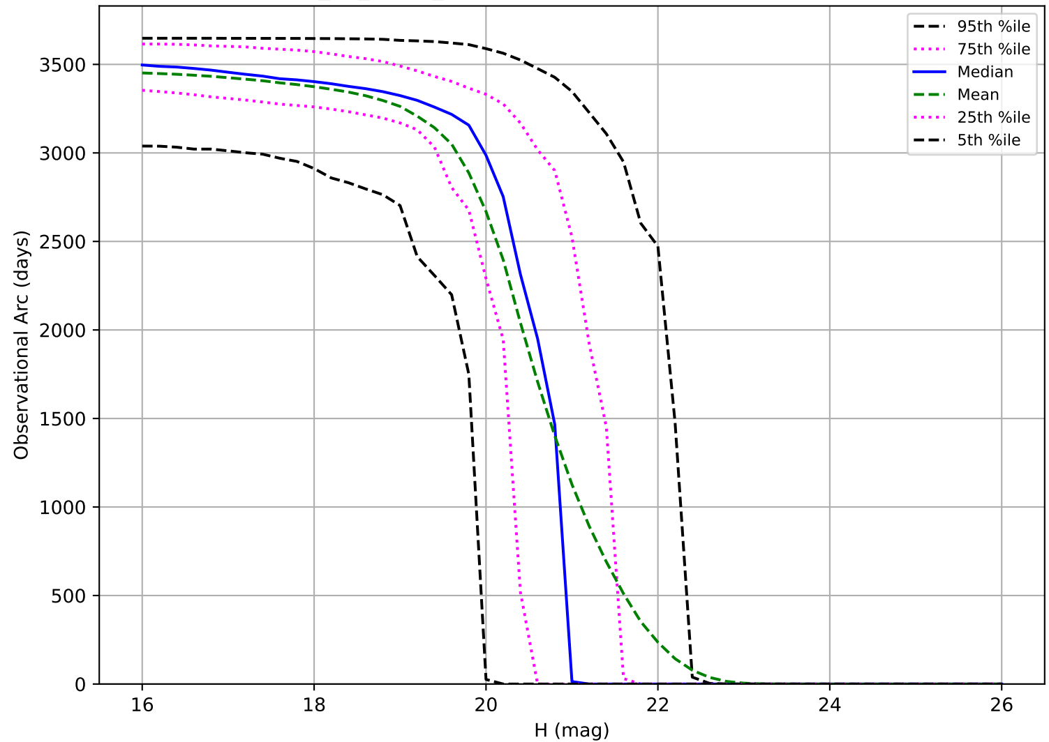
too_10_4v3.4_10yrs: Observational Arc Length MBA
