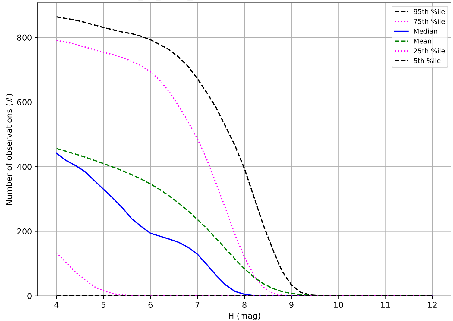
too_10_4v3.4_10yrs: Number of observations TNO
