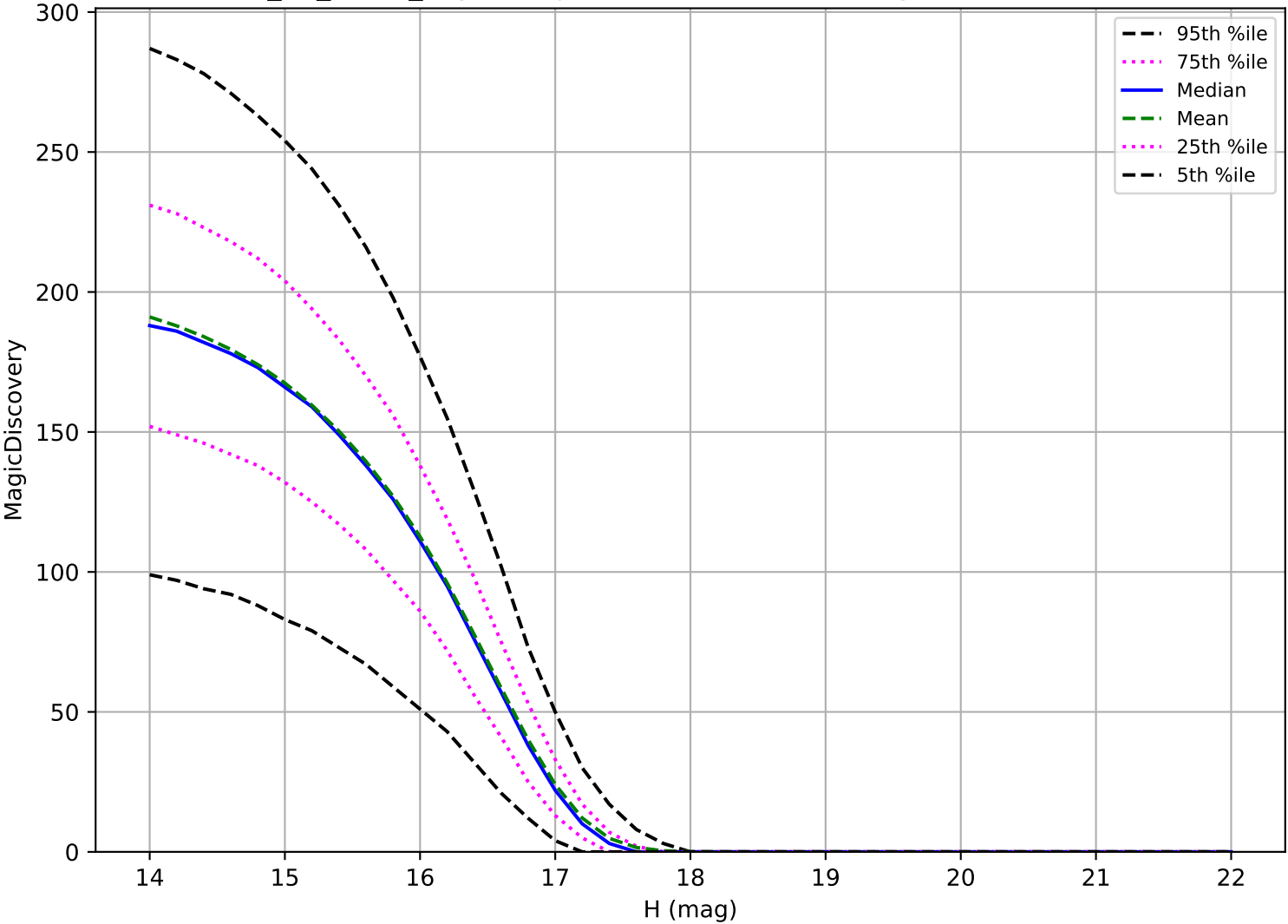
too_10_4v3.4_10yrs: Trojan 6 detections in 60 nights detection loss
