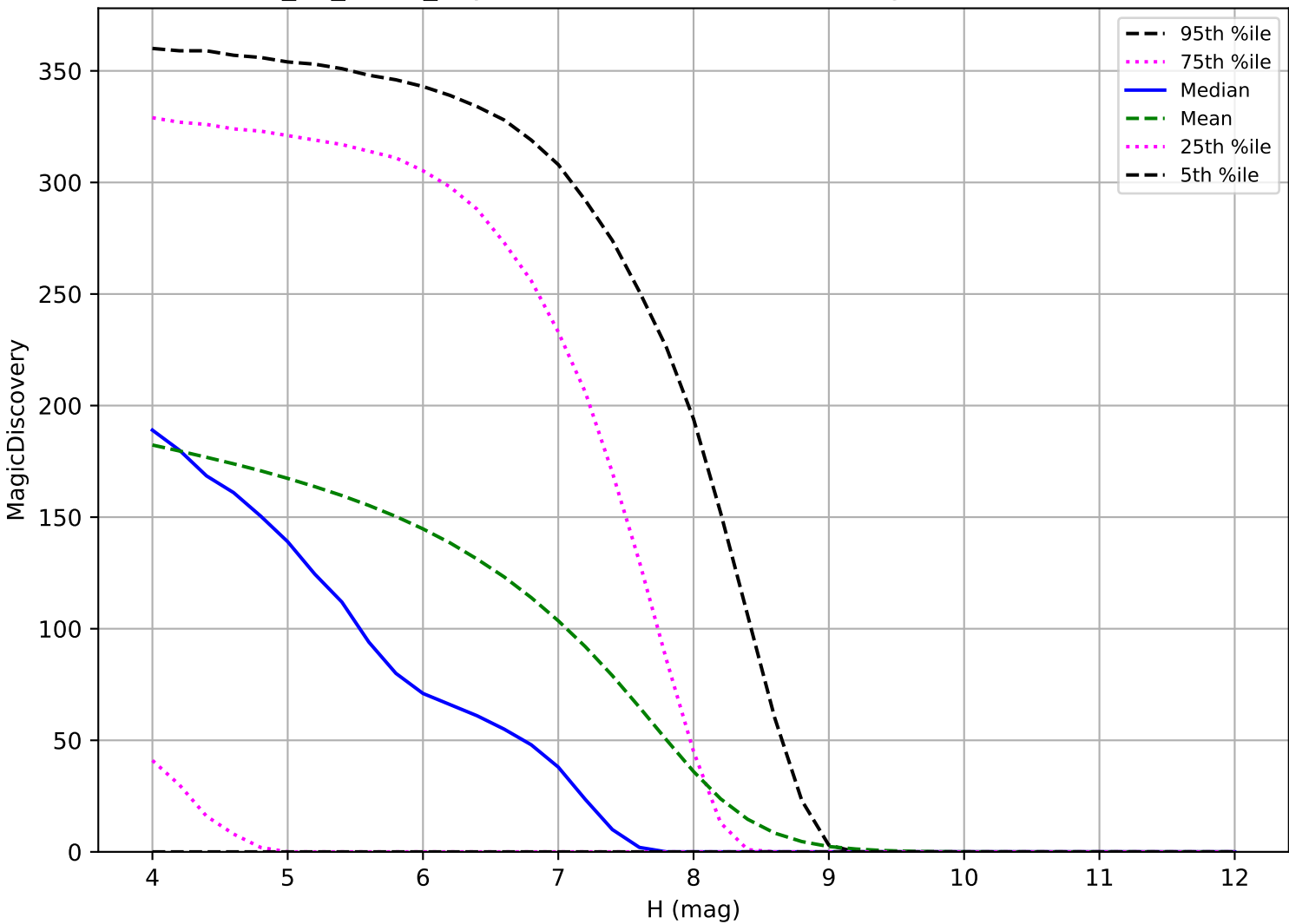
too_10_4v3.4_10yrs: TNO 6 detections in 60 nights detection loss
