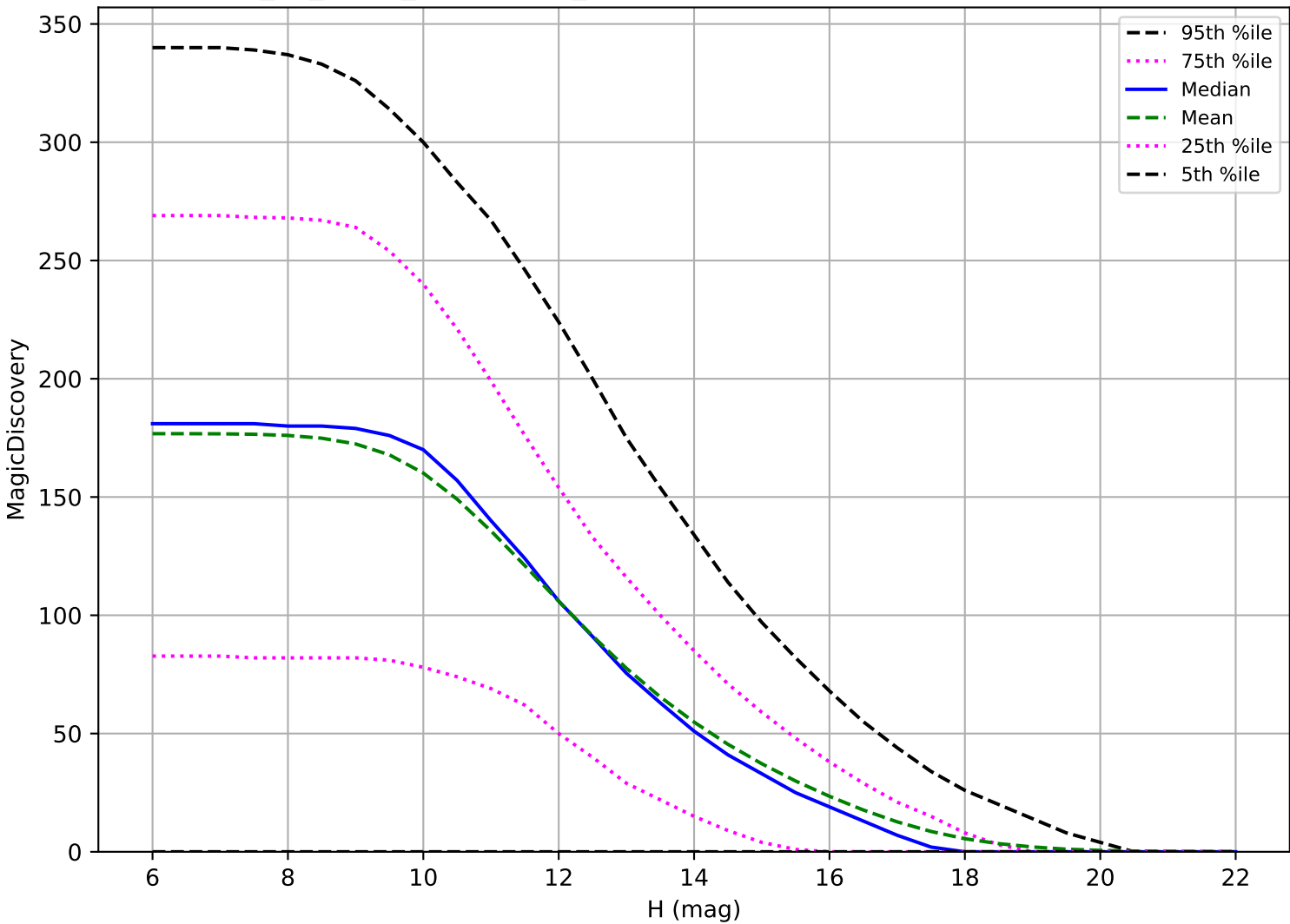
too_10_4v3.4_10yrs: OCC_r5 6 detections in 60 nights detection loss
