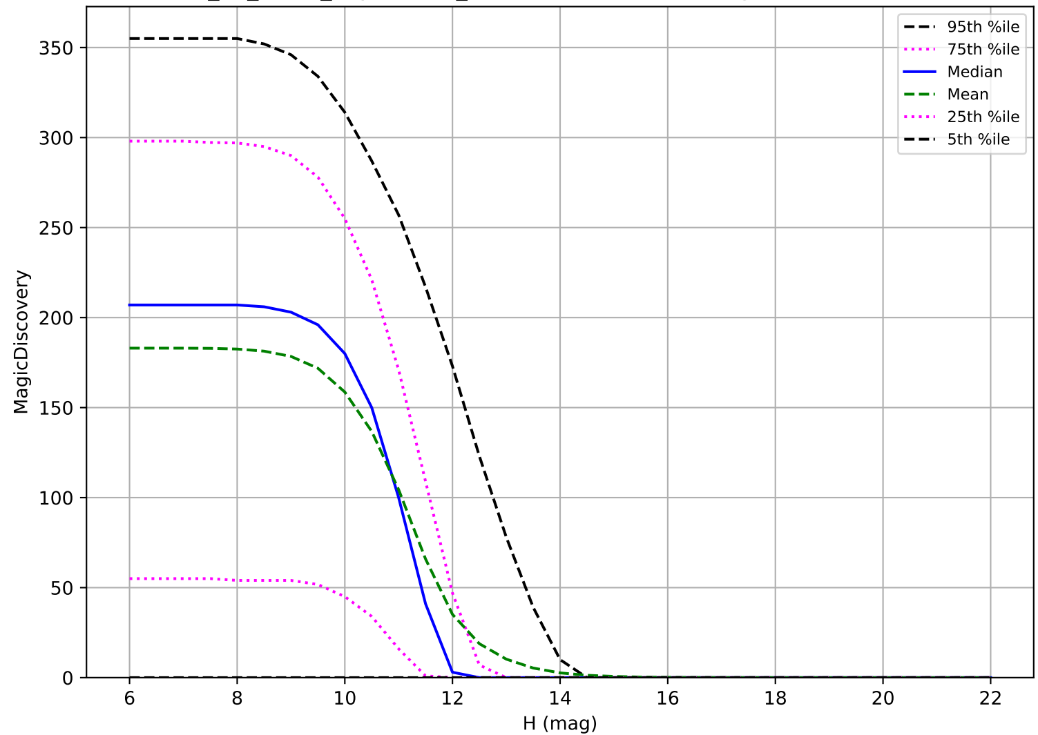
too_10_4v3.4_10yrs: OCC_r20 6 detections in 60 nights detection loss
