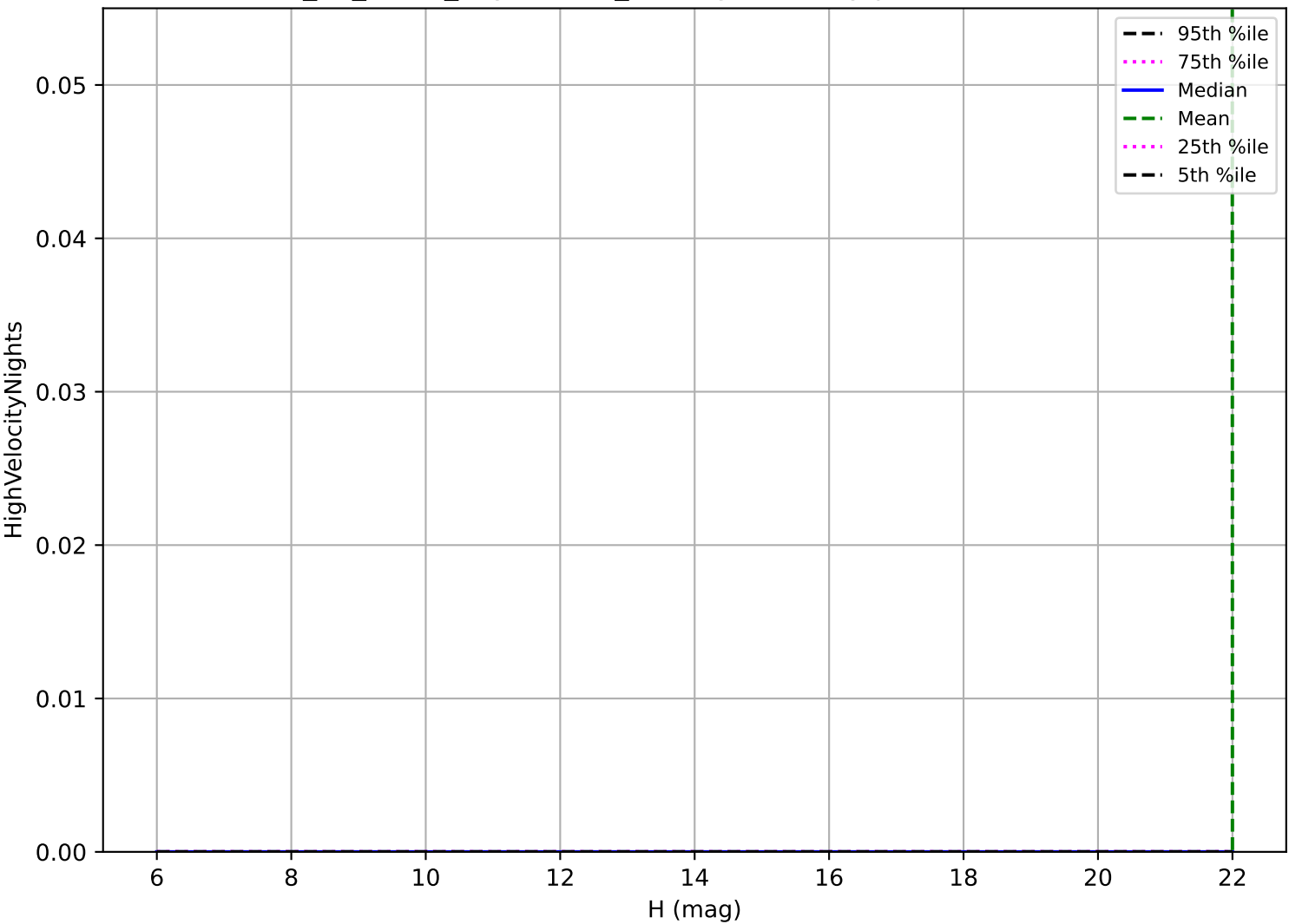
too_10_4v3.4_10yrs: OCC_r20 High velocity pair detection loss
