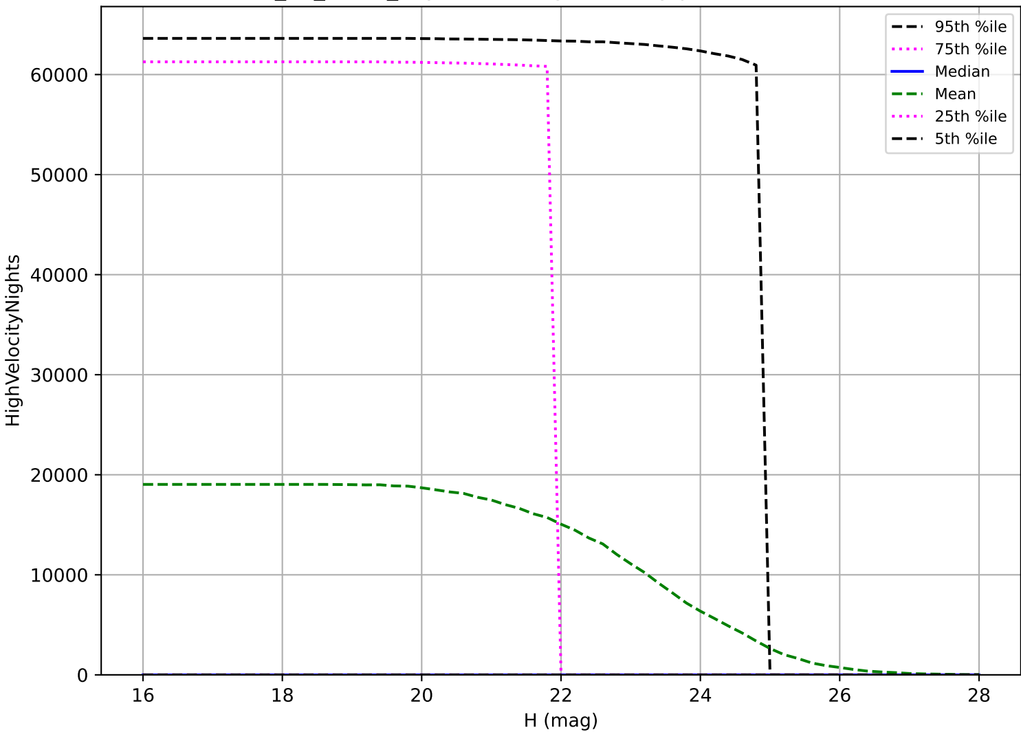
too_10_4v3.4_10yrs: NEO High velocity pair detection loss
