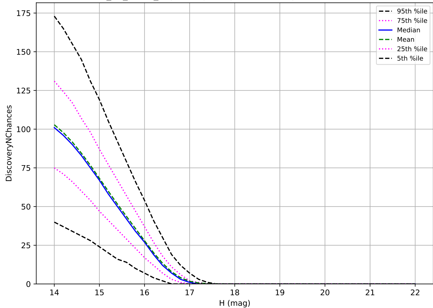
too_10_4v3.4_10yrs: Trojan 3 pairs in 15 nights detection loss
