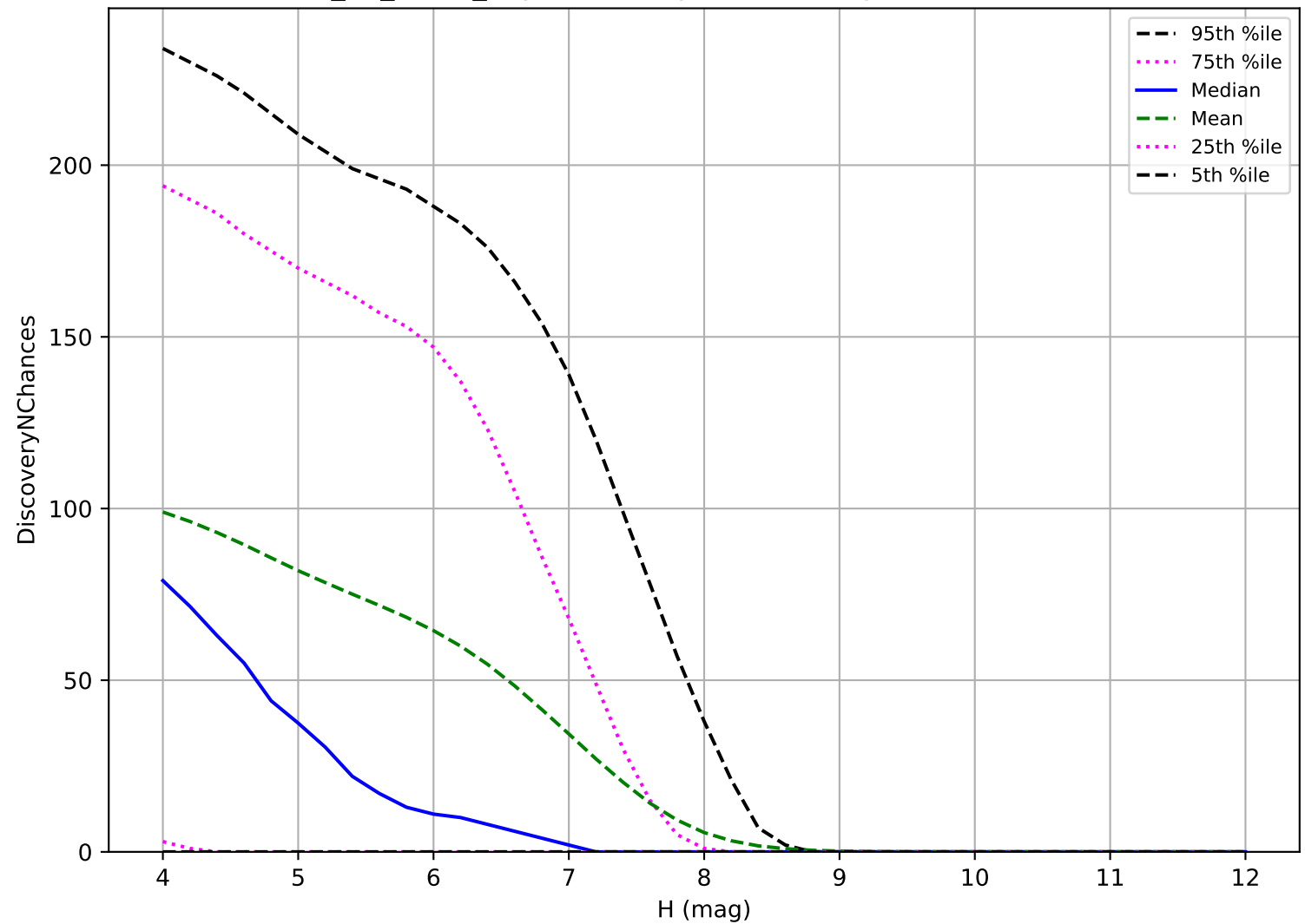
too_10_4v3.4_10yrs: TNO 3 pairs in 15 nights detection loss
