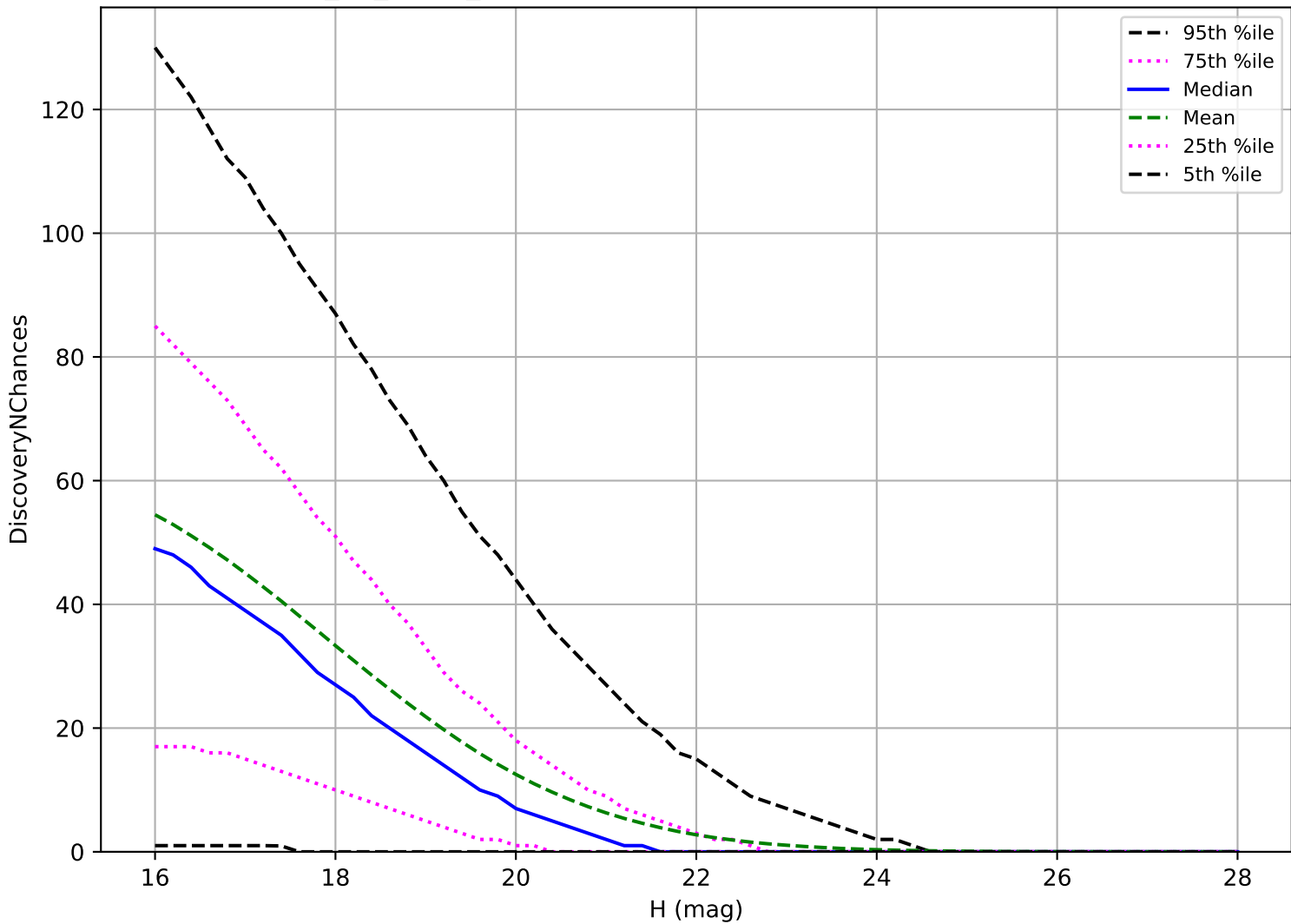
too_10_4v3.4_10yrs: PHA 3 pairs in 15 nights detection loss
