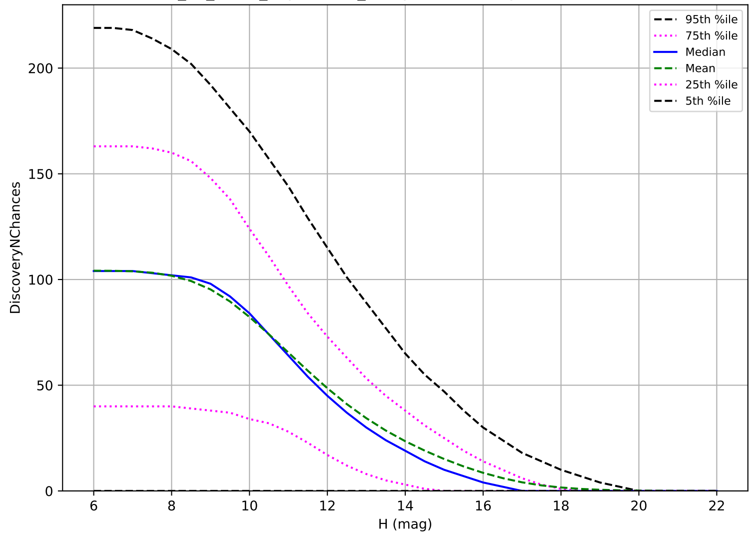
too_10_4v3.4_10yrs: OCC_r5 3 pairs in 15 nights detection loss
