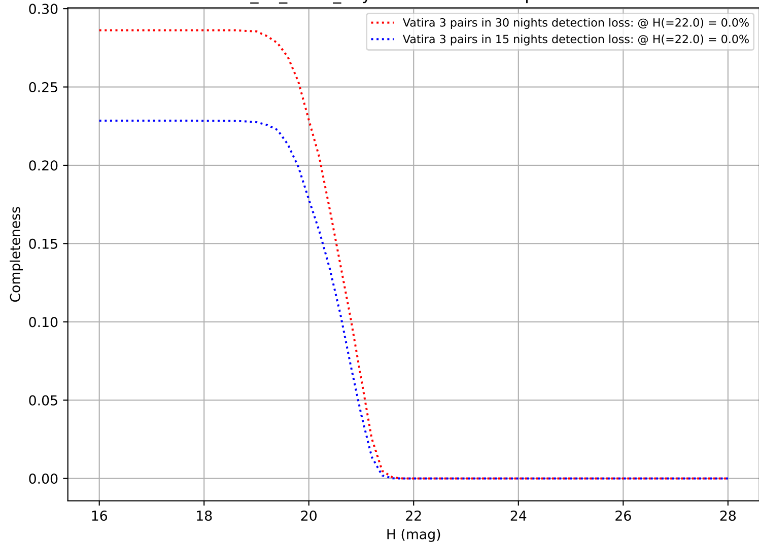
too_10_4v3.4_10yrs: DifferentialCompleteness
