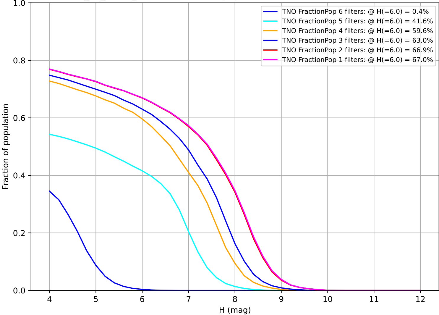
too_10_4v3.4_10yrs: Fraction of population with colors in X filters TNO
