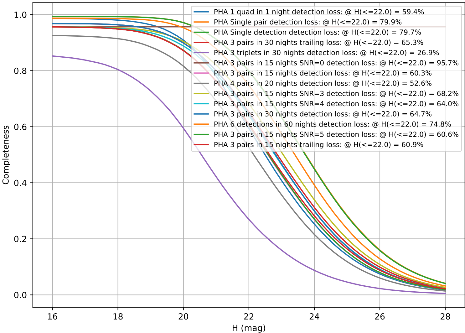
too_10_4v3.4_10yrs: CumulativeCompleteness
