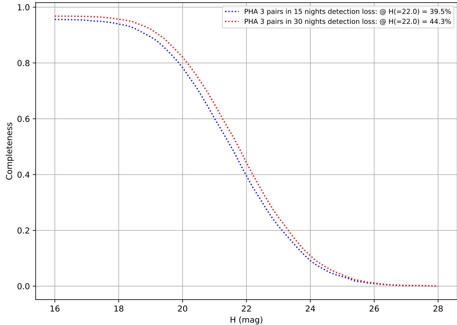
too_10_4v3.4_10yrs: DifferentialCompleteness
