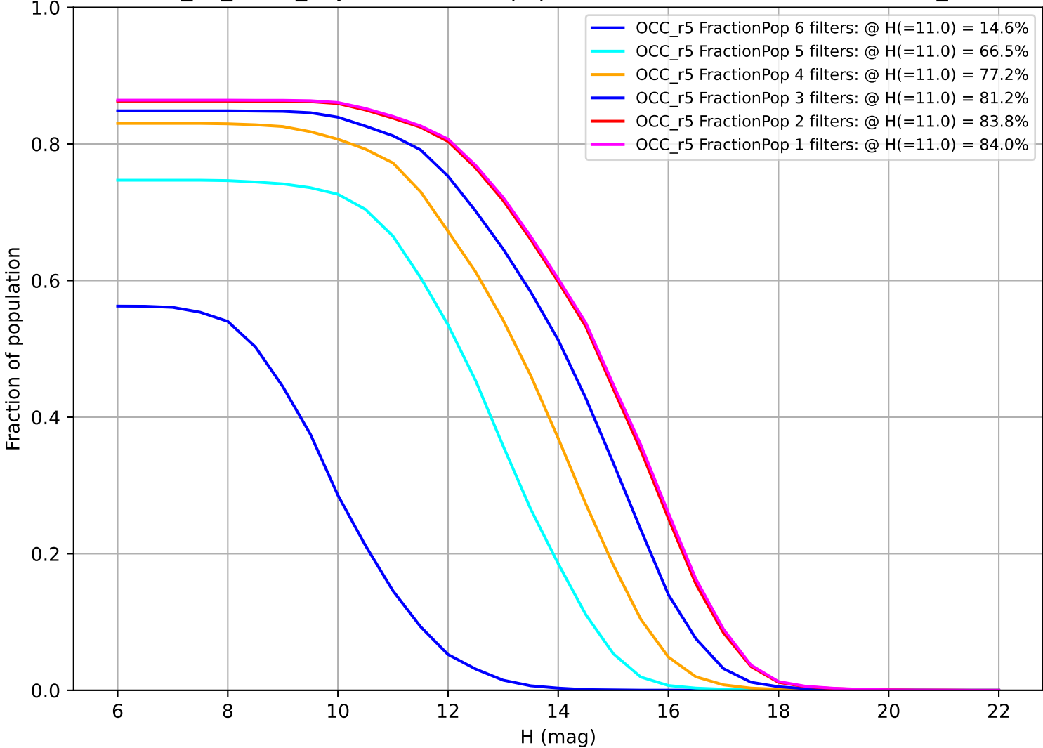
too_10_4v3.4_10yrs: Fraction of population with colors in X filters OCC_r5
