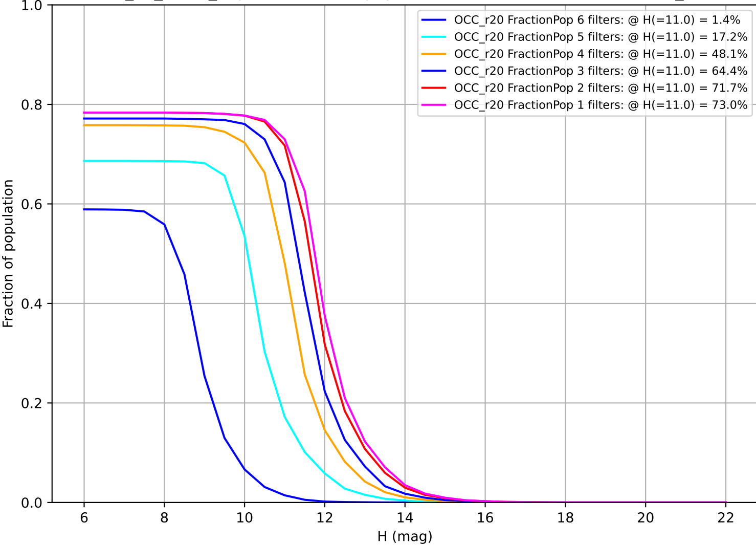
too_10_4v3.4_10yrs: Fraction of population with colors in X filters OCC_r20
