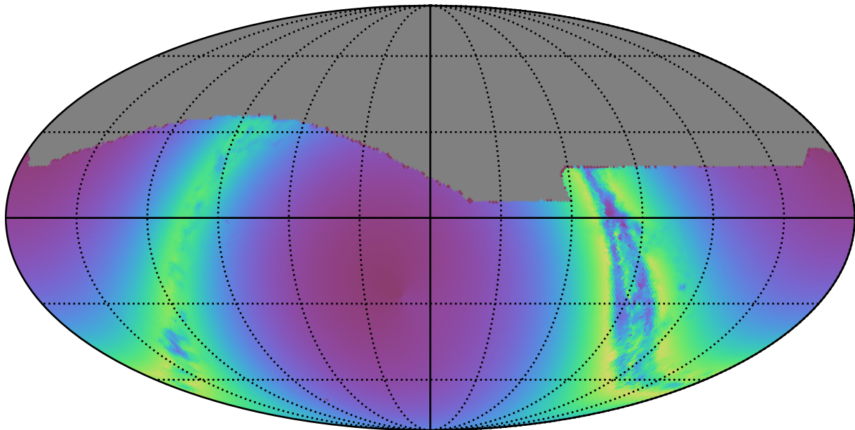
too_10_4v3.4_10yrs : young_stars
