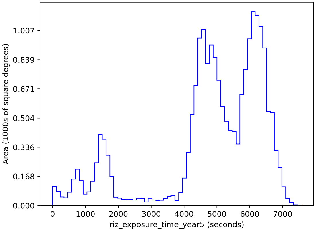
too_10_4v3.4_10yrs gri band non-DD: riz_exposure_time_year5
