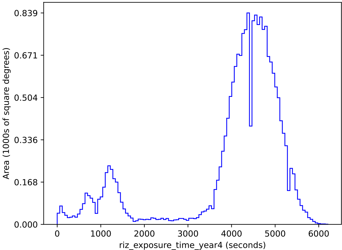
too_10_4v3.4_10yrs gri band non-DD: riz_exposure_time_year4
