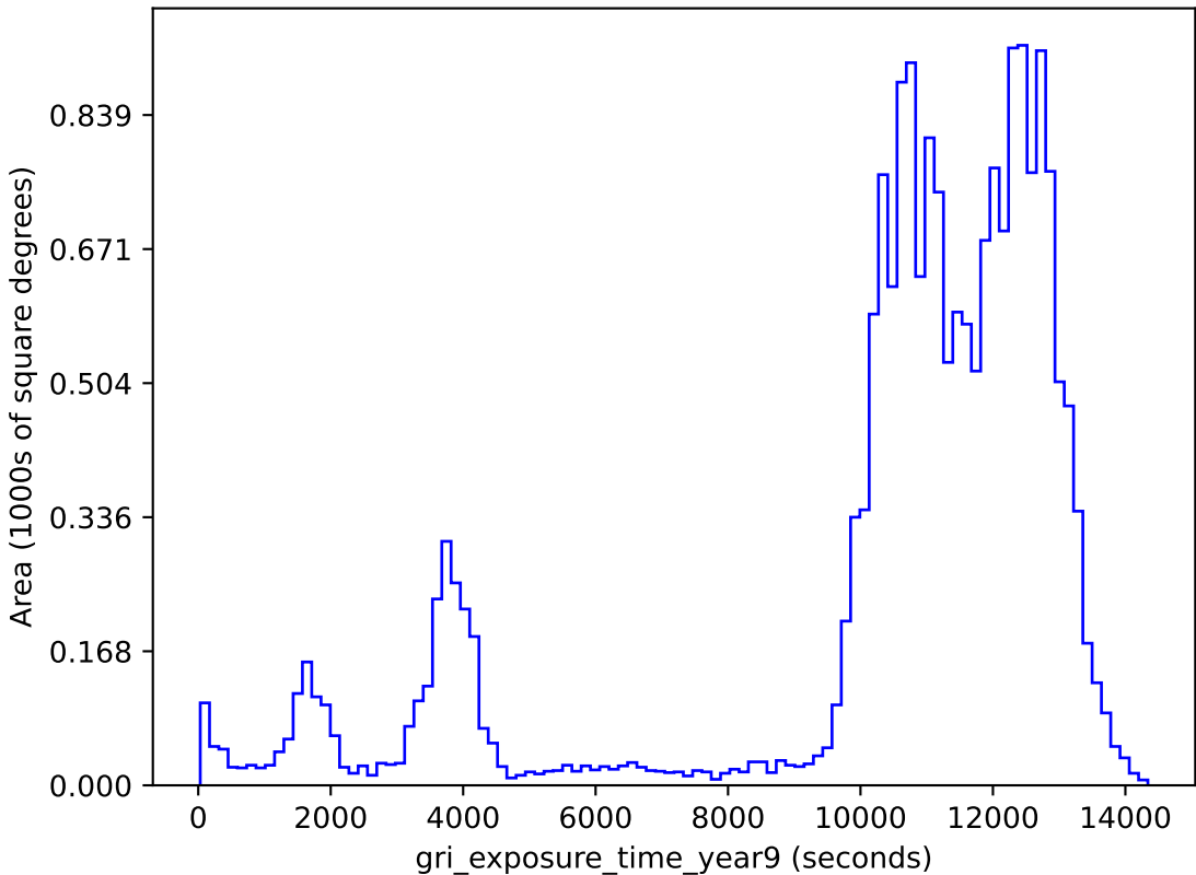
too_10_4v3.4_10yrs gri band non-DD: gri_exposure_time_year9
