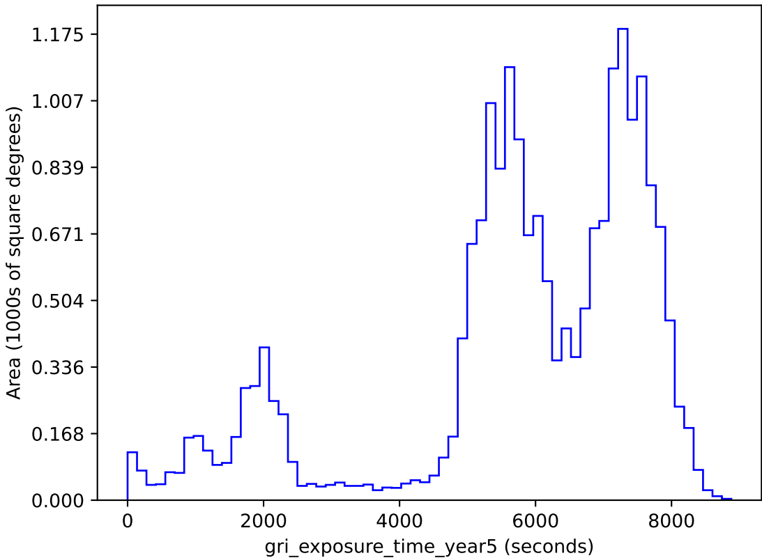
too_10_4v3.4_10yrs gri band non-DD: gri_exposure_time_year5
