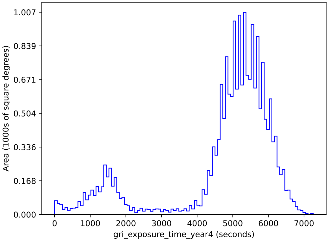
too_10_4v3.4_10yrs gri band non-DD: gri_exposure_time_year4
