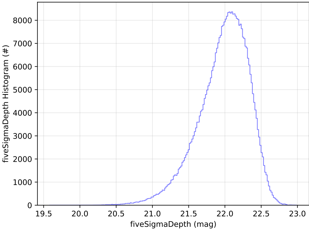
too_10_4v3.4_10yrs y: fiveSigmaDepth Histogram
