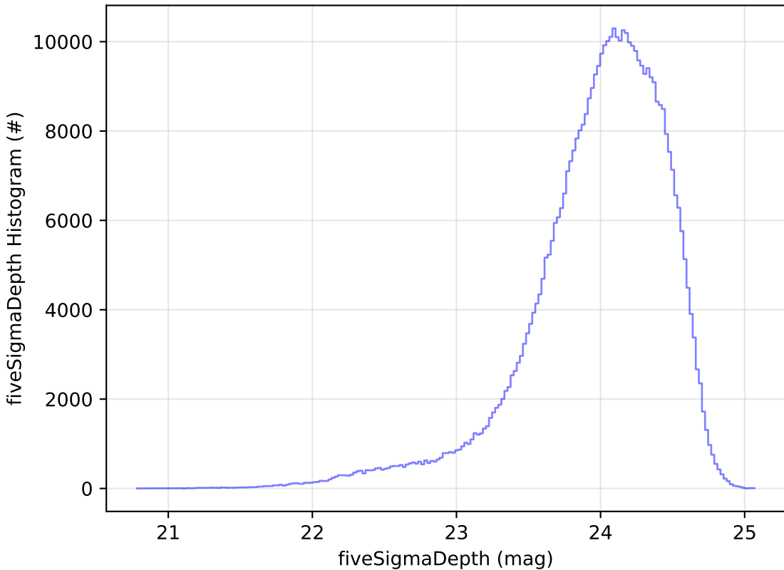
too_10_4v3.4_10yrs r: fiveSigmaDepth Histogram
