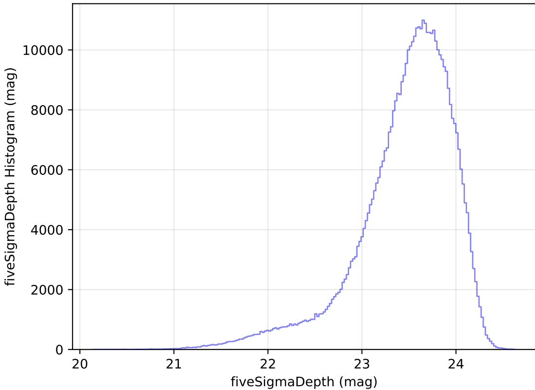
too_10_4v3.4_10yrs i: fiveSigmaDepth Histogram
