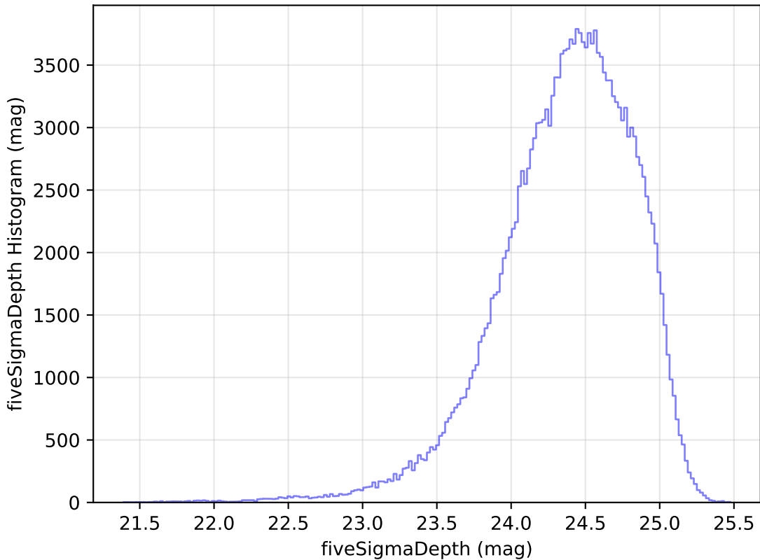
too_10_4v3.4_10yrs g: fiveSigmaDepth Histogram
